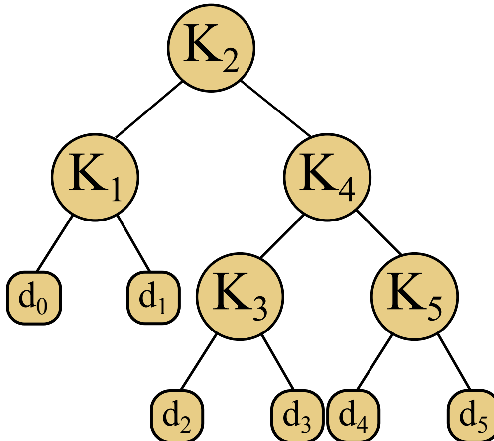
Optimal Binary Search Tree
